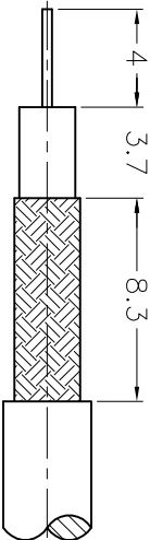
RECOMMENDED CABLE STRIPPING DIM'S (建議剝線尺寸)
